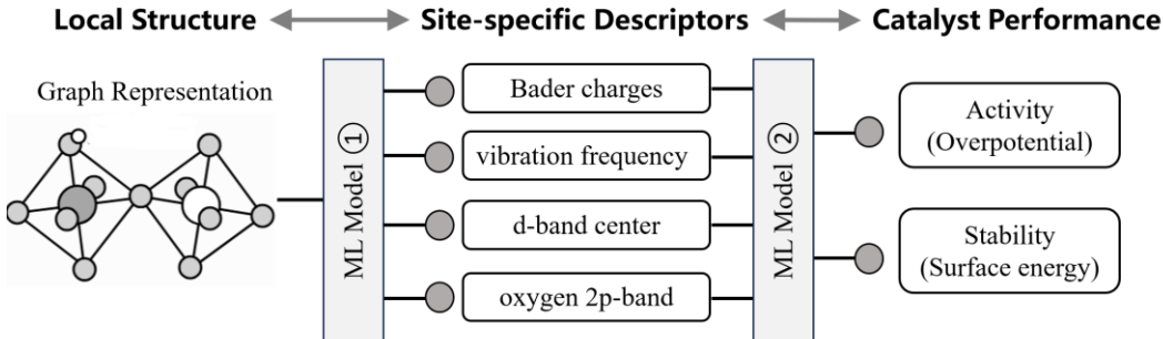
Figure 3 Machine learning mapping of local environment, per-site properties and catalyst performance
